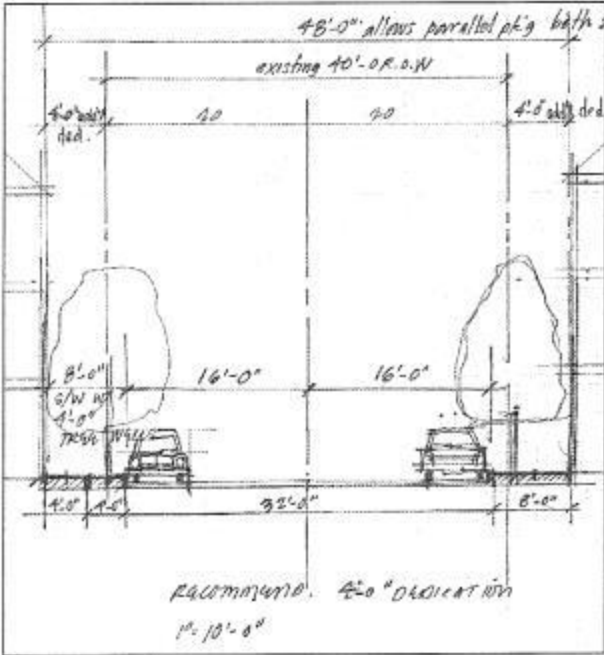
Figure 17.50.080-1: Typical local street.
